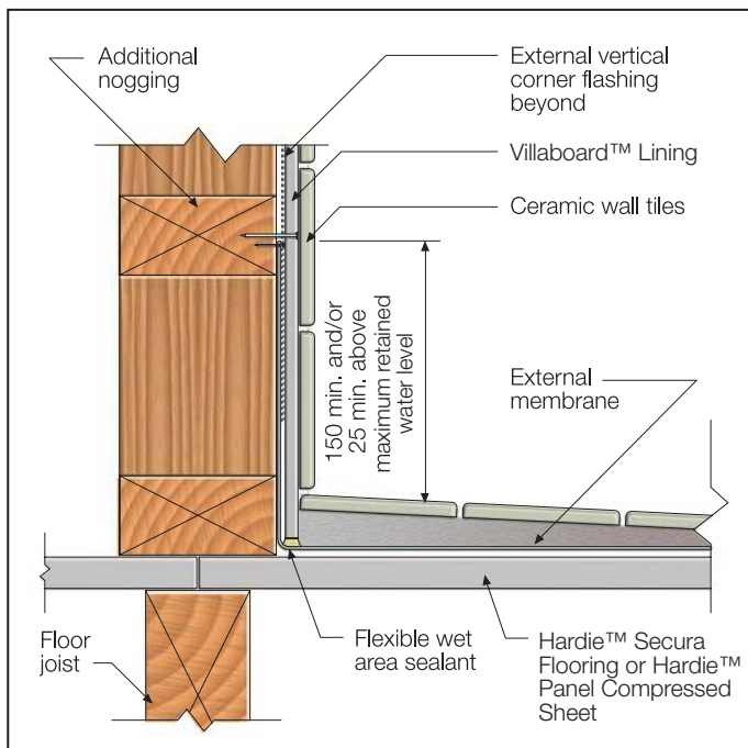
FIGURE 17 EXTERNAL MEMBRANE - VILLABOARD™ LINING
