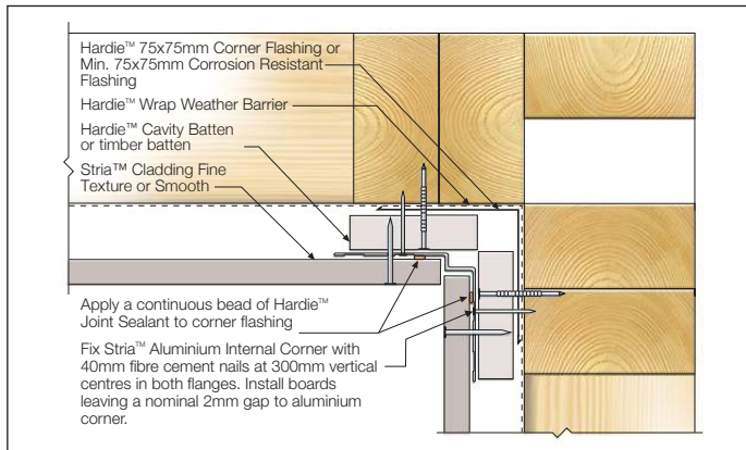
FIGURE 21 INTERNAL CORNER
