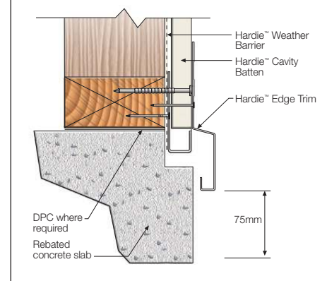
FIGURE 9B ALTERNATIVE SLAB EDGE DETAIL
