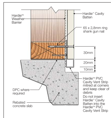
FIGURE 9A SLAB EDGE DETAIL
