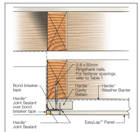
FIGURE 31 ABUTMENT DETAIL
