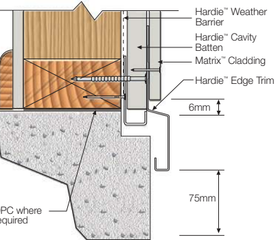
FIGURE 23 SLAB/EAVES DETAIL
