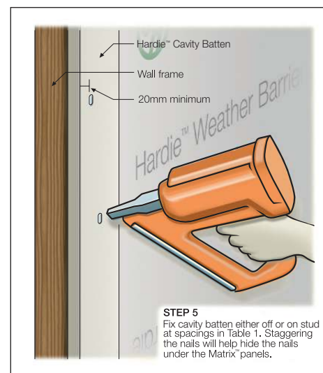
FIGURE 8 FIXING CAVITY BATTEN
