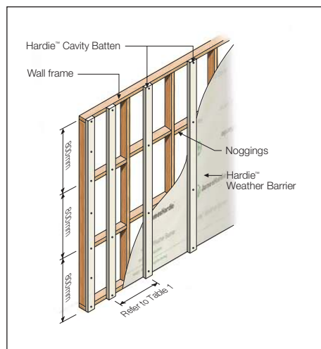
FIGURE 5 OFF-STUD FIXING
