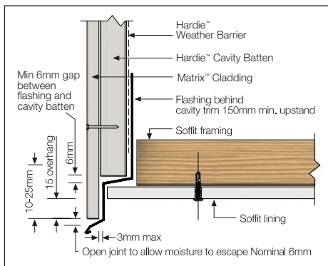
FIGURE 33 FACADE/SOFFIT JUNCTION
