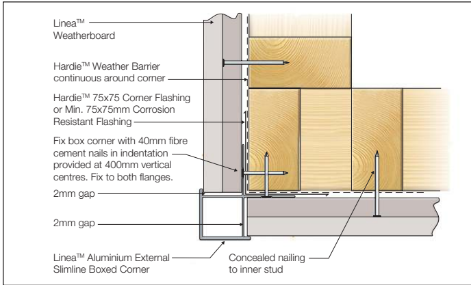
FIGURE 7 EXTERNAL SLIMLINE BOX CORNER DETAIL
