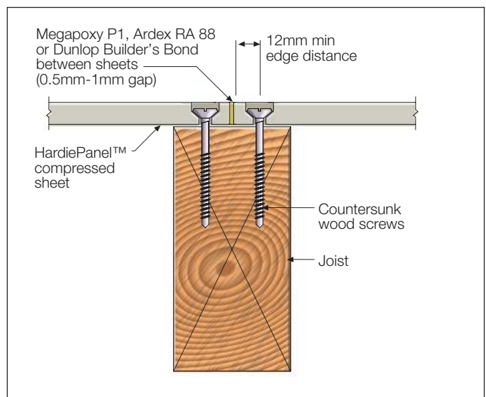
FIGURE 10 SCREW DETAIL
