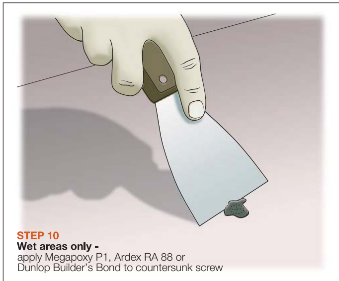
FIGURE 13 APPLY EPOXY
