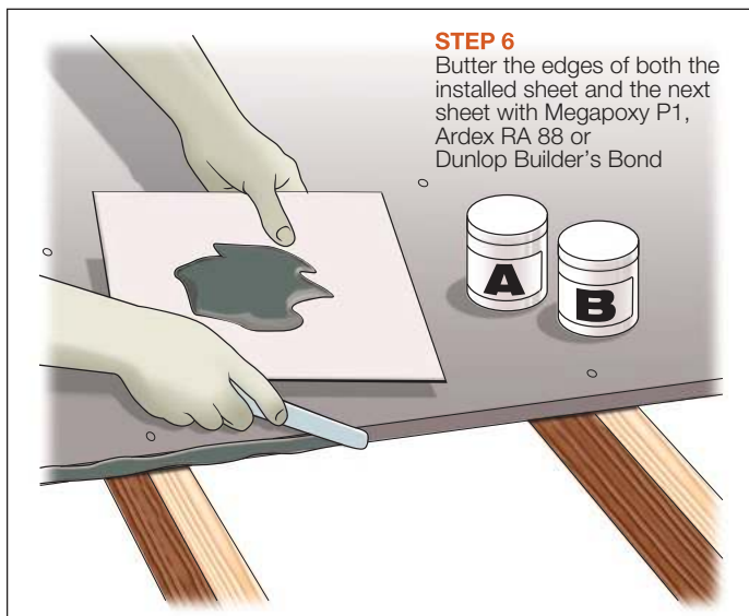
FIGURE 8 APPLYING EPOXY
