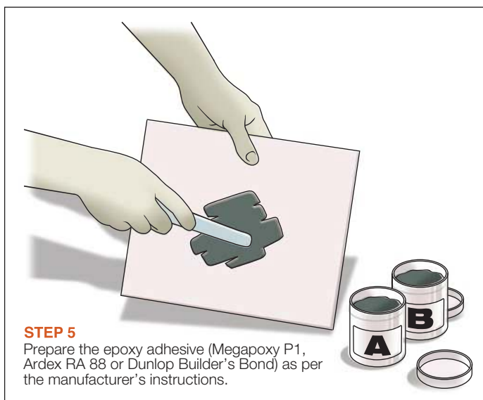
FIGURE 7 MIXING EPOXY
