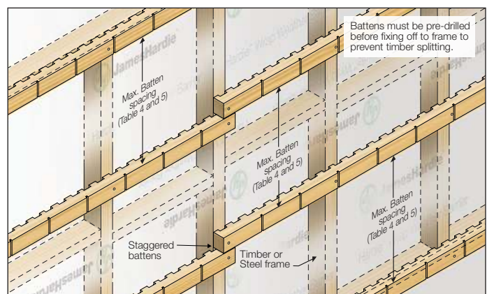
FIGURE 14 ON-STUD STAGGERED JOINTING OF BATTENS
