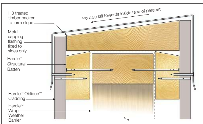
FIGURE 15 PARAPET DETAIL
