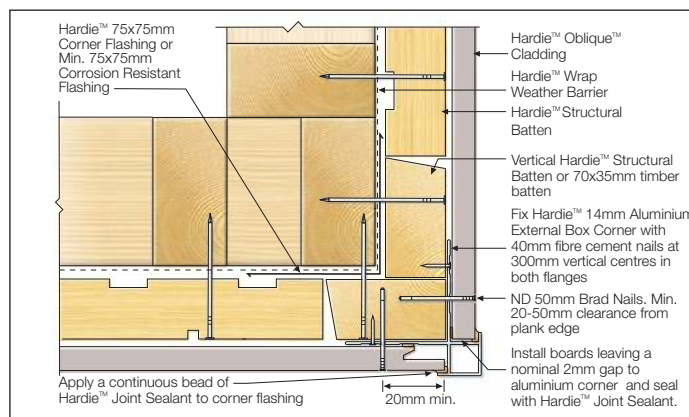
FIGURE 7 EXTERNAL BOX CORNER
