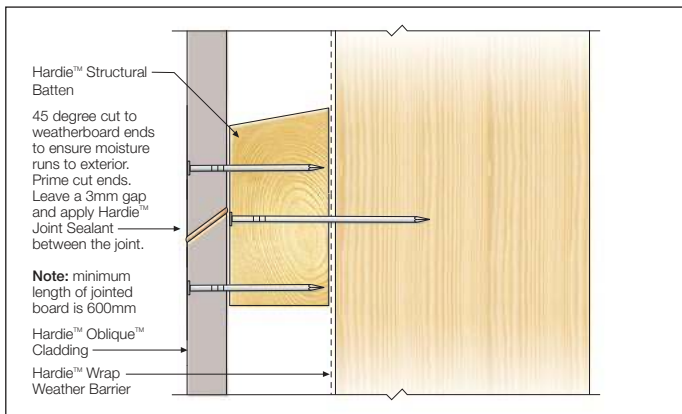
FIGURE 9 VERTICAL BUTT JOINT DETAIL
