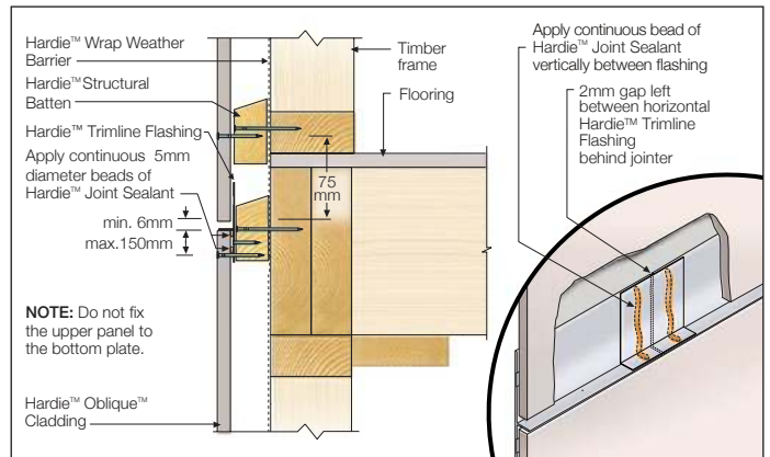
FIGURE 2 UPPER FLOOR JUNCTION
