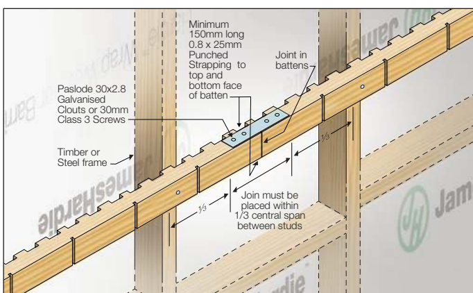
FIGURE 11 OFF-STUD JOINTING OF BATTENS - OPTION 2
