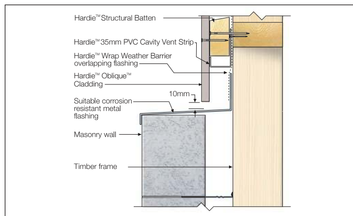
FIGURE 3 HORIZONTAL JUNCTION
