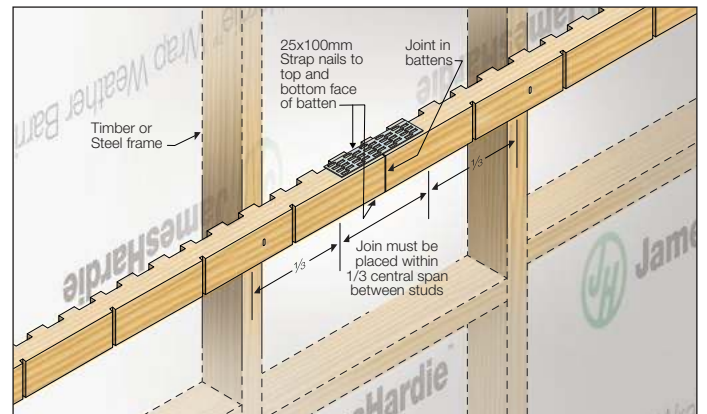
FIGURE 10 OFF-STUD JOINTING OF BATTENS - OPTION 1
