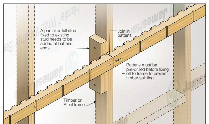
FIGURE 12 ON-STUD JOINTING OF BATTENS
