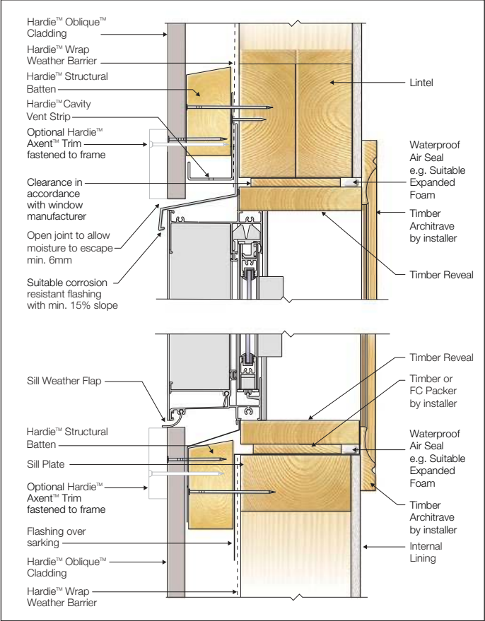
FIGURE 16 WINDOW HEAD AND SILL - TRIM
