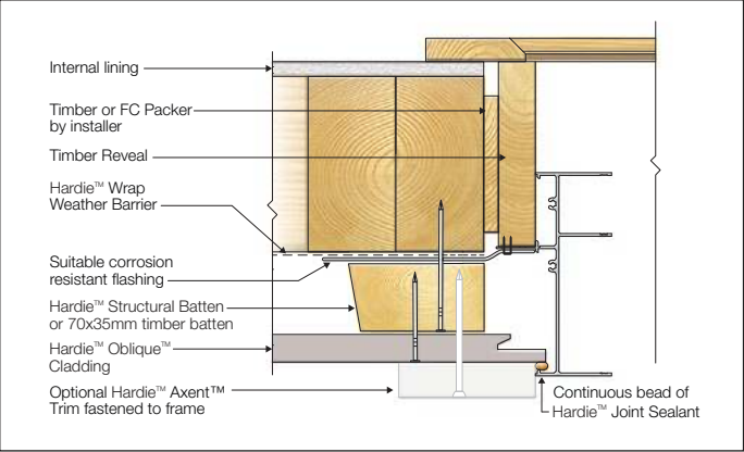
FIGURE 17 WINDOW JAMB - TRIM
