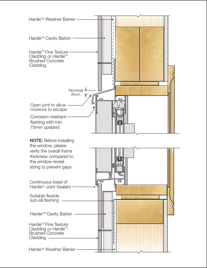
FIGURE 35 WINDOW HEAD AND SILL - CAVITY BATTEN
