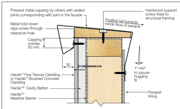
FIGURE 27 PARAPET CAPPING DETAIL
