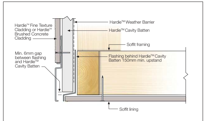
FIGURE 28 FACADE/SOFFT JUNCTION
