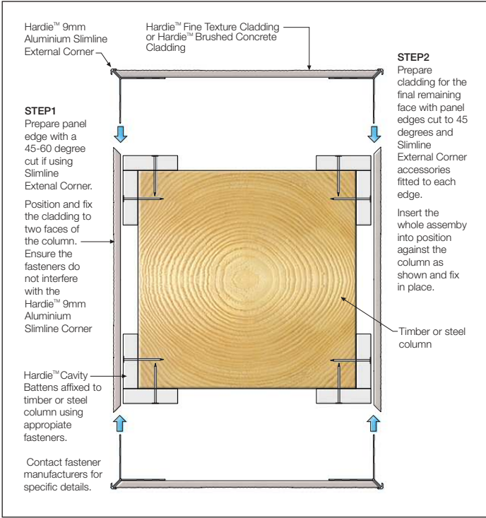
FIGURE 40 FIXING TO TIMBER OR STEEL COLUMN
