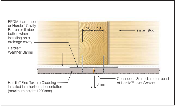
FIGURE 38 VERTICAL BUTT JOINT DIRECT FIX
