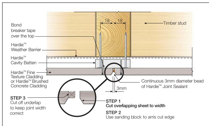
FIGURE 29 VERTICAL BUTT JOINT
