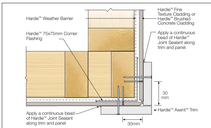
FIGURE 14 TRIM CORNER OPTION
