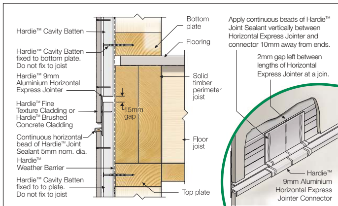
FIGURE 25 FLOOR LEVEL JUNCTION HORIZONTAL EXPRESS JOISTER
