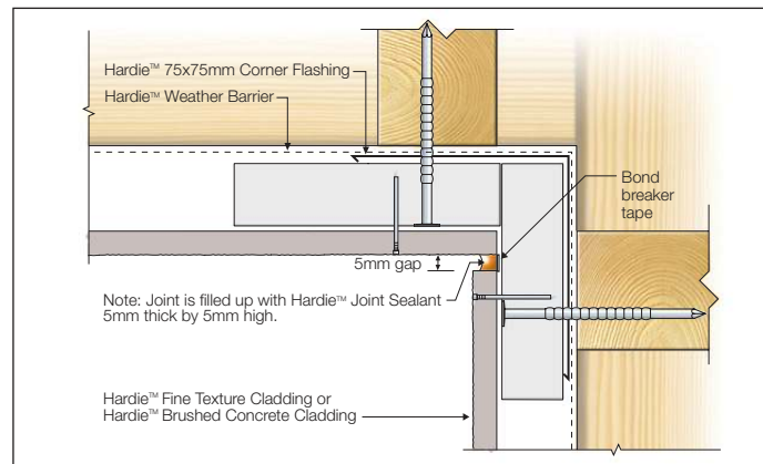
FIGURE 34 SEALANT FILL OPTION - CAVITY BATTEN
