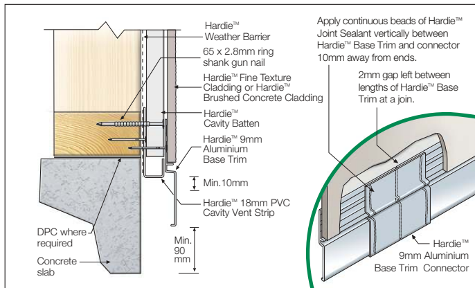
FIGURE 23 SLAB EDGE DETAIL
