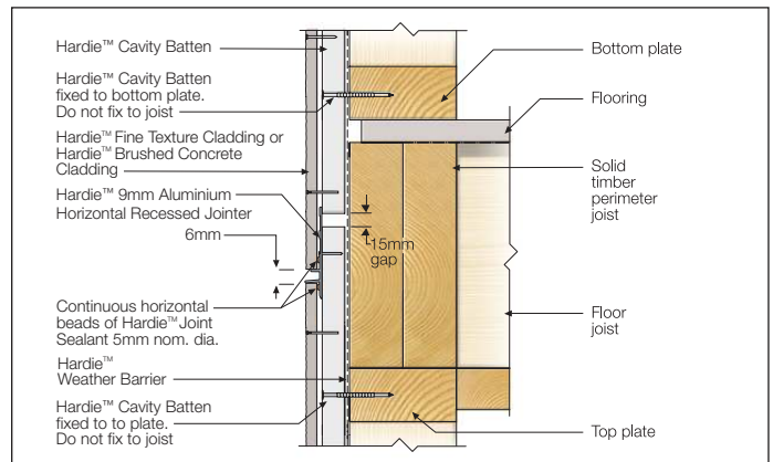
FIGURE 26 FLOOR LEVEL JUNCTION HORIZONTAL RECESSED JOISTER OPTION
