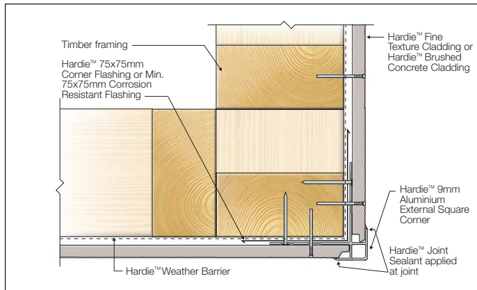
FIGURE 12 ALUMINIUM SQUARE CORNER OPTION
