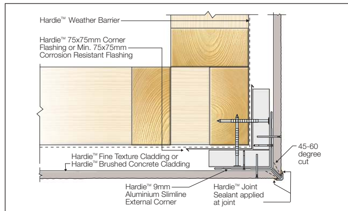
FIGURE 31 SLIM CORNER OPTION - CAVITY BATTEN
