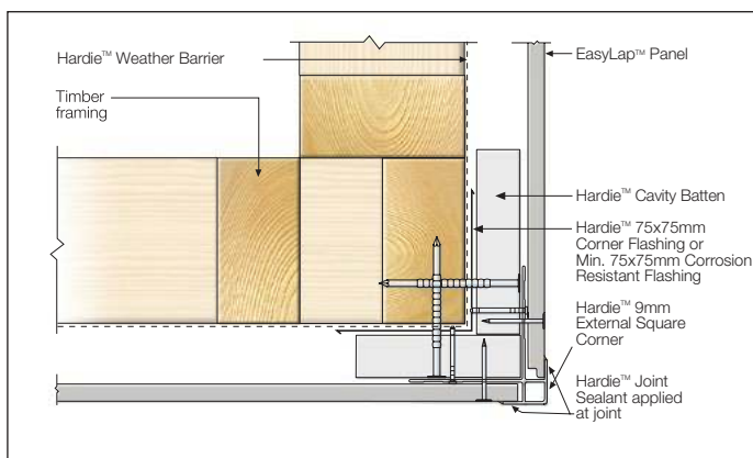
FIGURE 21 ALUMINIUM BOX CORNER OPTION - CAVITY BATTEN
