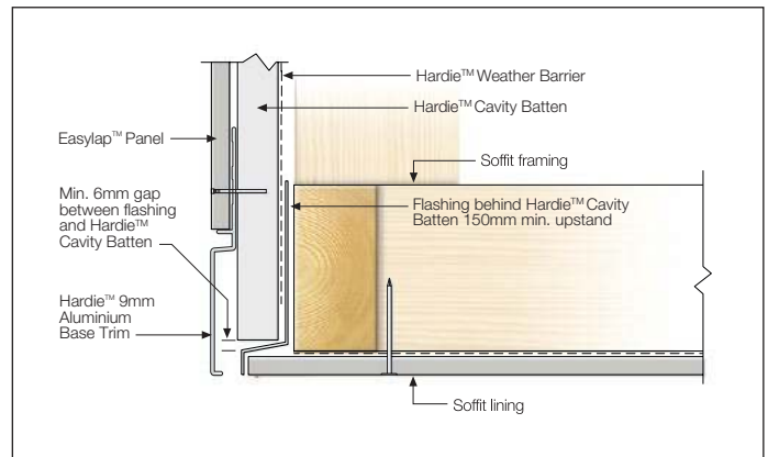
FIGURE 20 FACADE/SOFFIT JUNCTION
