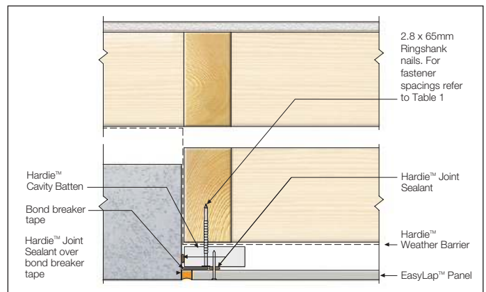
FIGURE 18 ABUTMENT DETAIL
