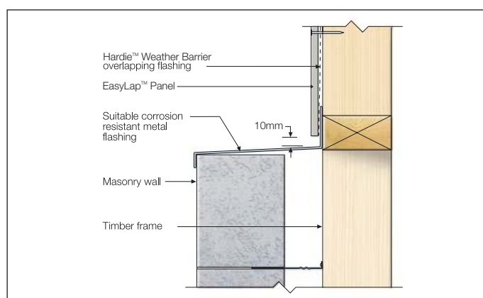
FIGURE 4 HORIZONTAL JUNCTION
