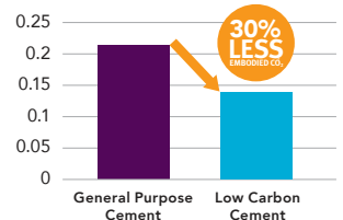
Embodied CO 2 of 25MPa Concrete (tonnes CO 2 / m 3 )
